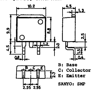
Case Outline—[2069] unit: mm
