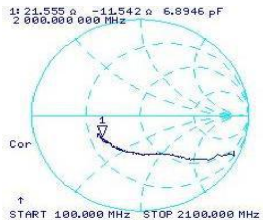
S22e -FREQUENCY
