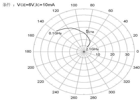
S21e -FREQUENCY
