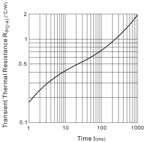
Fig.6 Thermal resistance
