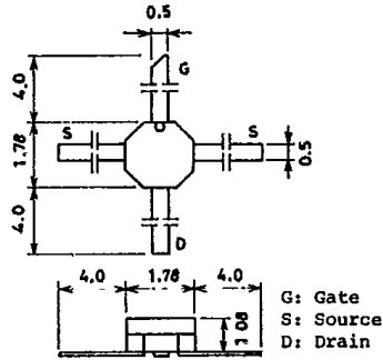
Case Outline—[2072] unit: mm
