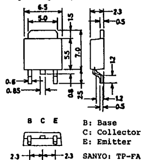
Case Outline—[2044] unit: mm
