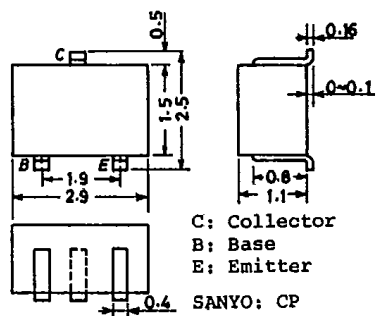
Case Outline—[2018A] unit: mm
