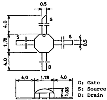
Case Outline—[2071] unit: mm
