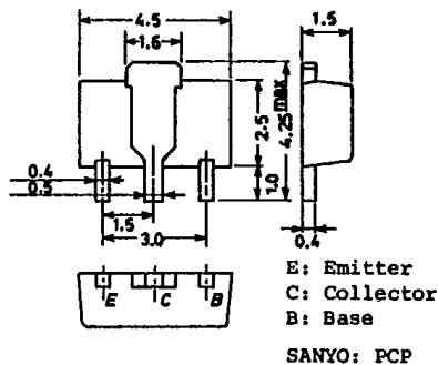
Case Outline—[2038] unit: mm
