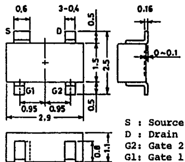
Case Outline—[2046] unit: mm
