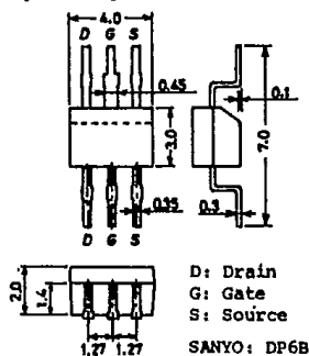
Case Outline—[2028A] unit: mm
