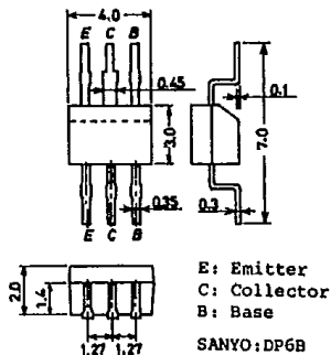
Case Outline—[2030A] unit: mm
