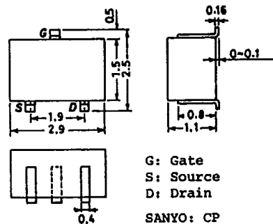
Case Outline—[2050] unit: mm
