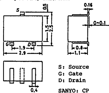
Case Outline—[2024A] unit: mm
