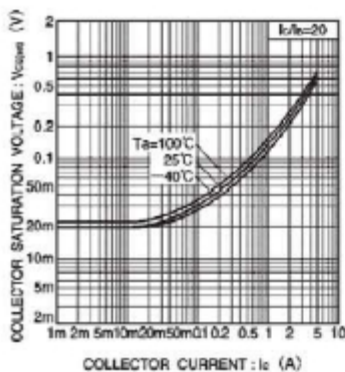
Fig.7 Collector-emitter saturation voltage vs. collector current (III)
