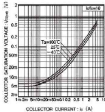
Fig.5 Collector-emitter saturation voltage vs. collector current (I)
