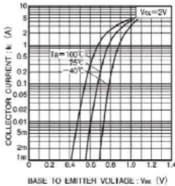
Fig.1 Grounded emitter propagation characteristics
