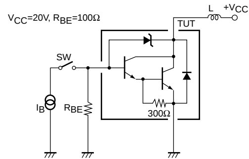
Es/b Test Circuit
