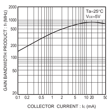
Fig.6 Gain bandwidth product vs. collector current
