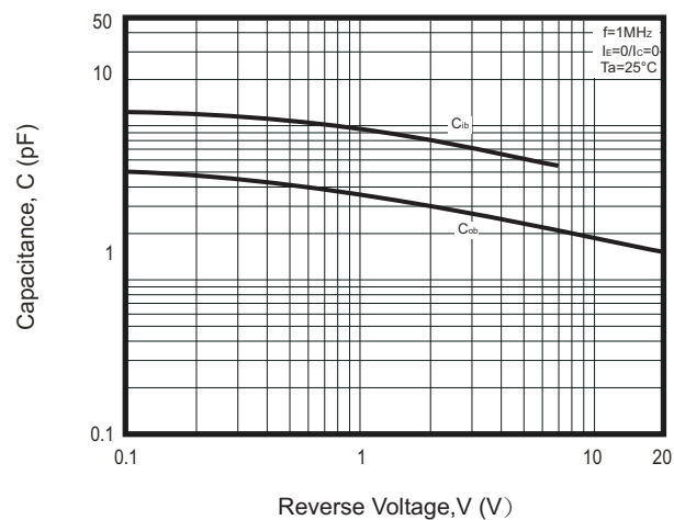
Fig.7- C_{ob}/C_{ib} \text{ --- } V_{CE}/V_{EB}
