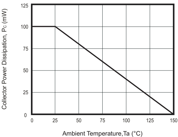
Fig.8 - P_c \text{ --- } T_a
