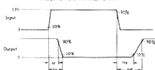
RESPONSE WAVEFORM
