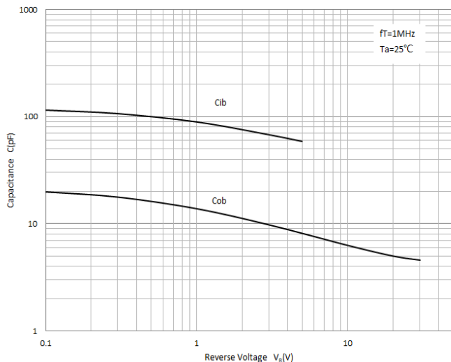
C_{ob}/C_{ib}-V_{CB}/V_{EB}
