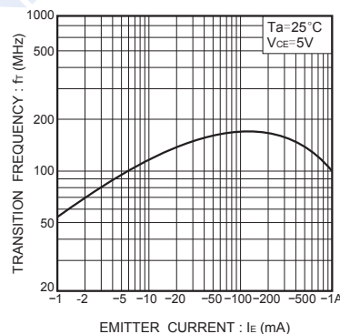
Fig.6 Transition frequency vs. emitter current
