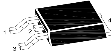
1. Base 2. Collector 3. Emitter 4. Collector TO-252 Plastic Package
