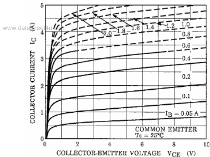
Fig.3 Static Characteristic
