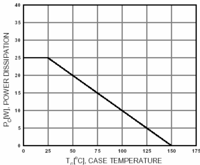
Fig.7 Power Derating
