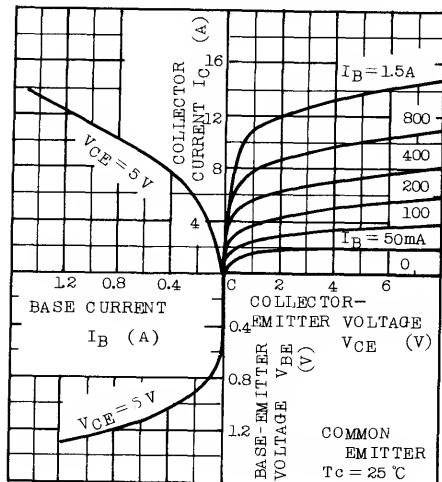
STATIC CHARACTERISTICS
