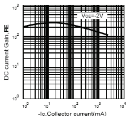
Fig.7 DC current gain
