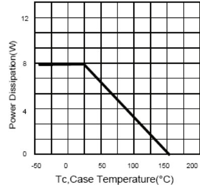
Fig.3 Power Derating
