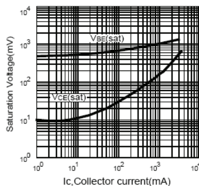
Fig.8 Saturation Voltage
