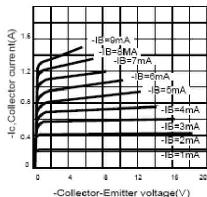
Fig.1 Static characteristics
