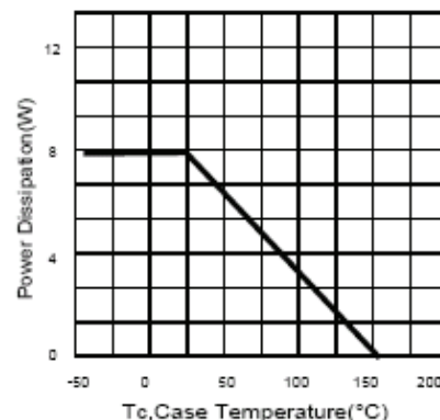
Fig.3 Power Derating
