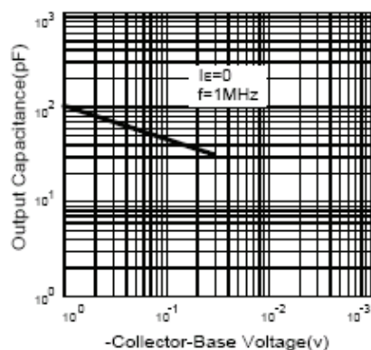
Fig.4 Collector Output capacitance
