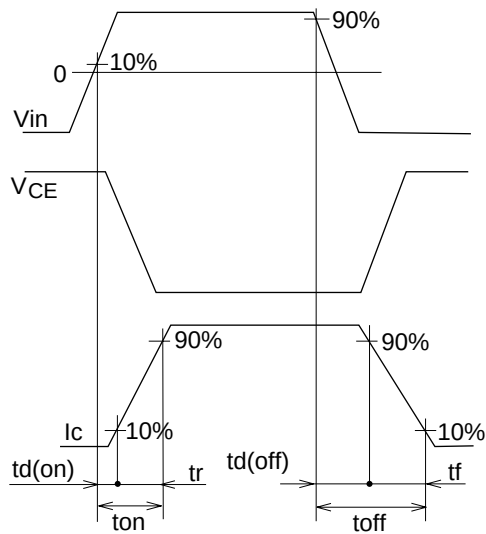
Waveforms
