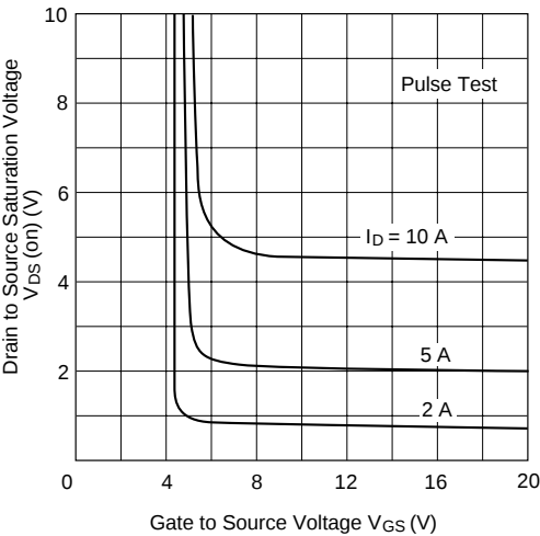
Drain to Source Stauration Voltage vs. Gate to Source Voltage
