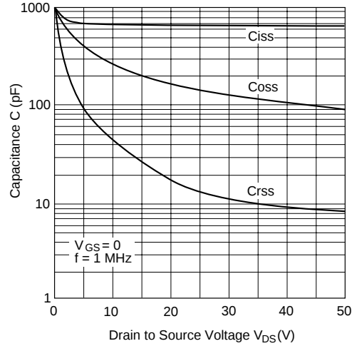
Typical Capacitance vs. Drain Source Voltage
