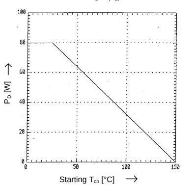
Power Dissipation
