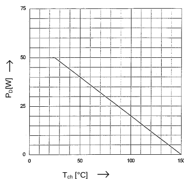
Power Dissipation
