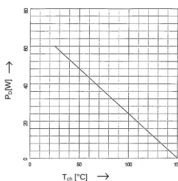
Power Dissipation
