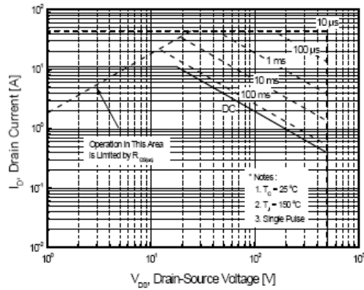
Fig.9 Maximum Safe Operation Area
