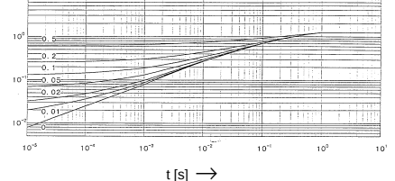
Transient Thermal impedance
