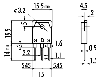
TO-3P
