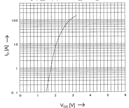
Typical Transfer Characteristics I_D = f(V_{GS}) ; 80μs pulse test; V_{DS} = 25V ; T_{ch} = 25^\circ\text{C}
