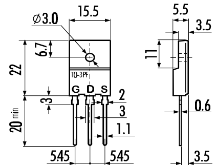
TO-3PF
