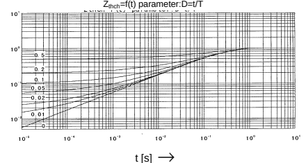
Transient Thermal Impedance Z_{\theta ch} = f(t) parameter: D = t/T
