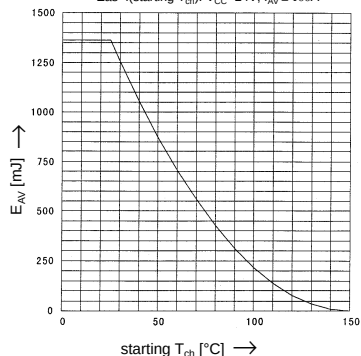
Maximum Avalanche Energy vs. starting T_{ch} E_{as} = f(\text{starting } T_{ch}) ; V_{CC} = 24V ; I_{AV} \leq 100A
