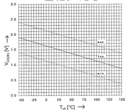
Gate Threshold Voltage vs. T_{ch} V_{GS(th)} = f(T_{ch}) ; I_D = 1mA ; V_{DS} = V_{GS}
