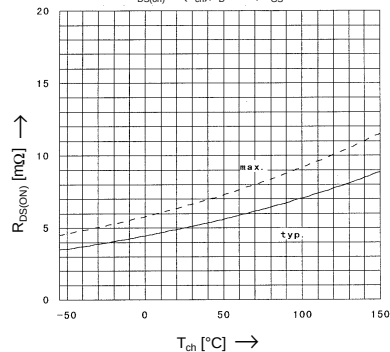
Drain-Source On-State Resistance vs. T_{ch} R_{DS(on)} = f(T_{ch}) ; I_D = 50A ; V_{GS} = 10V
