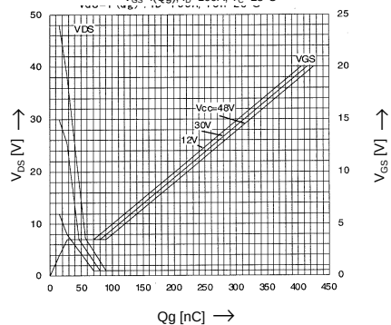
Typical Gate Charge Characteristic V_{GS} = f(Q_g) ; I_D = 100A ; T_C = 25^\circ\text{C}
