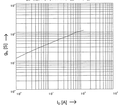
Typical Forward Transconductance vs. I_D g_{fs} = f(I_D) ; 80μs pulse test; V_{DS} = 25V ; T_{ch} = 25^\circ\text{C}
