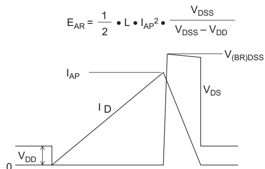
Avalanche Waveform
