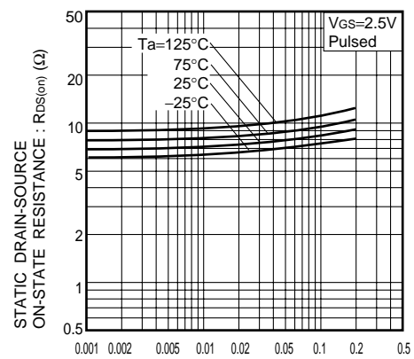
FIG. 6 STATIC DRAIN-SOURCE ON-STATE RESISTANCE V.S DRAIN CURRENT
