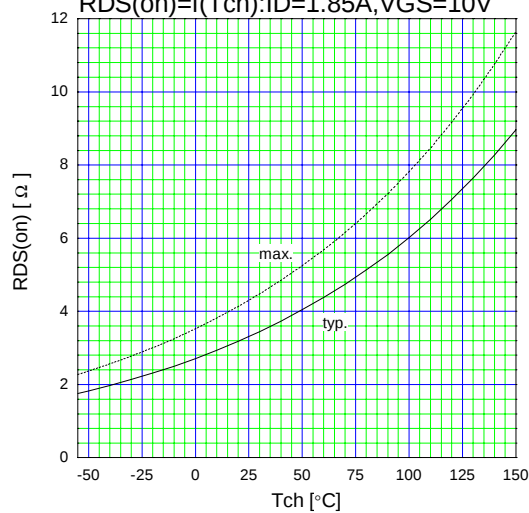
Drain-Source On-state Resistance R_{DS(on)}=f(T_{ch}): ID=1.85A , V_{GS}=10V
