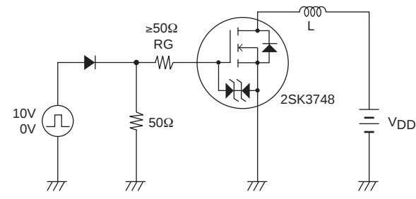
Fig.2 Switching Time Test Circuit
