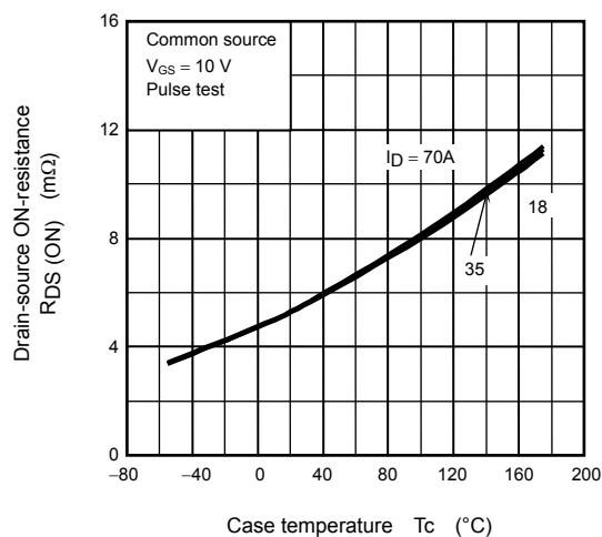
R_{DS(ON)} - T_c
