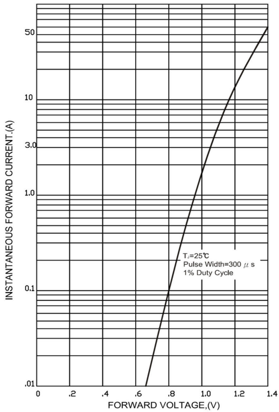
FIG.3-TYPICAL FORWARD CHARACTERISTICS
