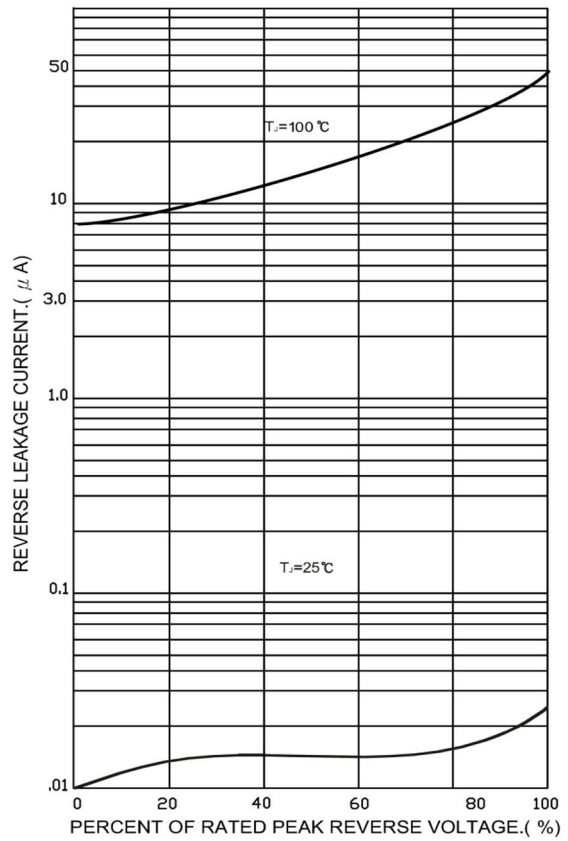
FIG.4-TYPICAL REVERSE CHARACTERISTICS
