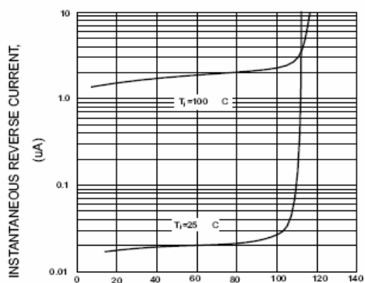
FIG.4-TYPICAL REVERSE CHARACTERISTICS PER BRIDGE ELEMENT
