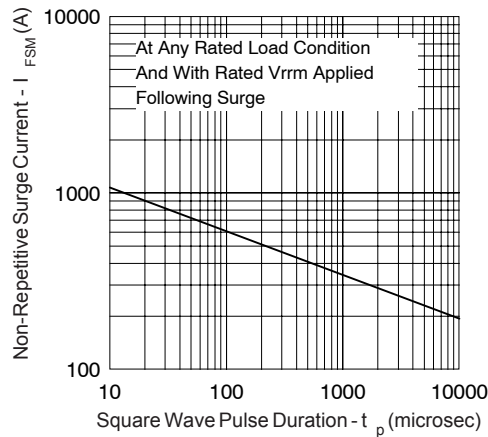
Fig. 7 - Max. Non-Repitive Surge Current (Per Leg)
