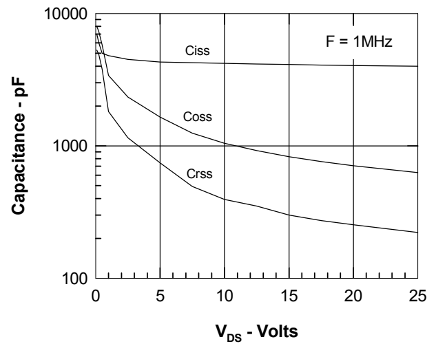
Figure 8. Capacitance Curves
