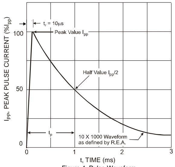
Figure 4. Pulse Waveform
