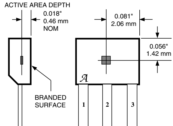
Dwg. MH-011-7
