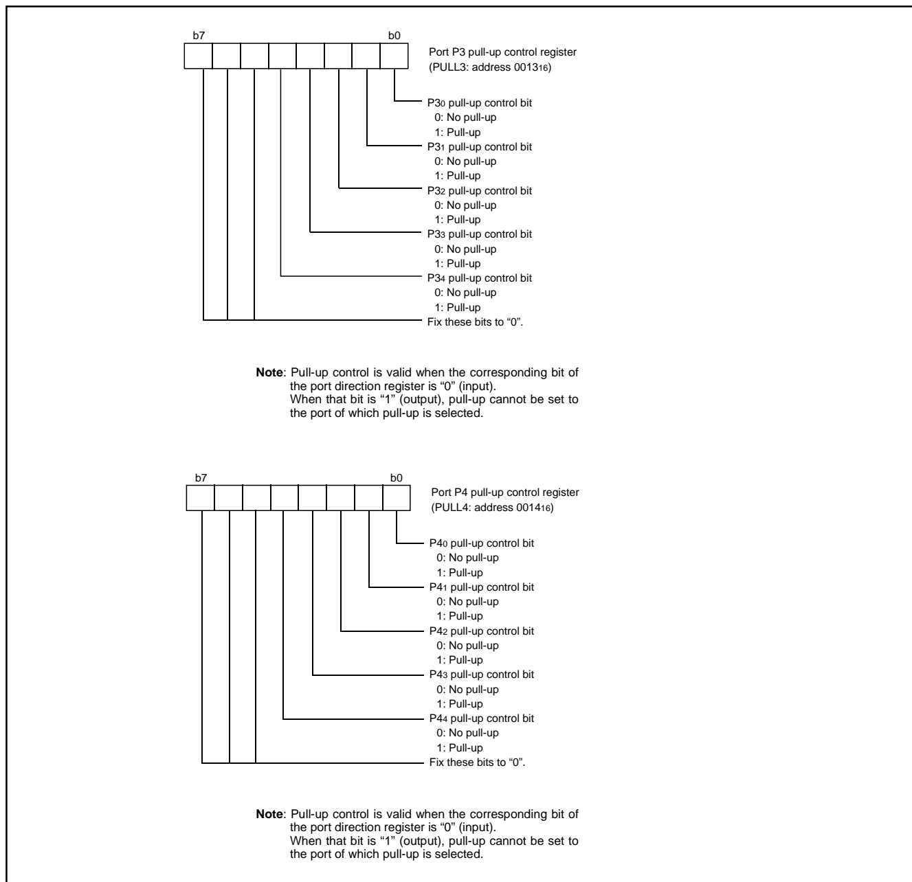
Fig. 14 Structure of port registers (2)
