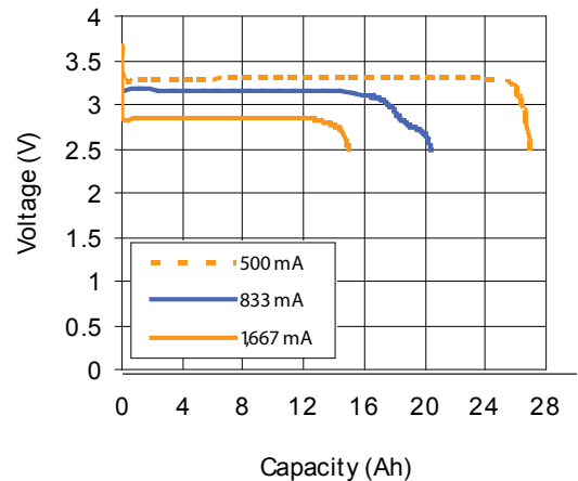
20°C discharge to 2.5 V
