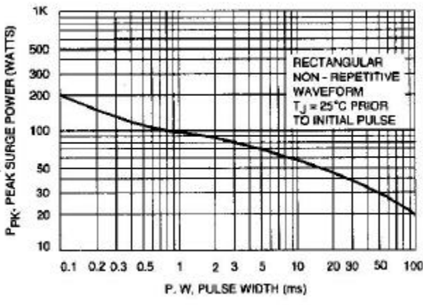
Fig. 3-MAXIMUM SURGE POWER
