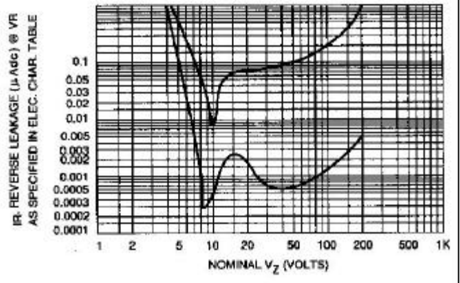
Fig. 4-TYPICAL REVERSE LEAKAGE
