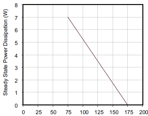
Figure 5. Steady Power Dissipation Derating Curve
