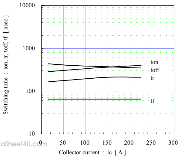
Switching time vs. Collector current (typ.) V_{cc}=600V, V_{GE}=\pm 15V, R_g=2.2\Omega, T_j=25^\circ C
