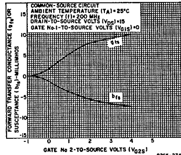
Fig. 6 - Y_{13} vs. V_{G2S}
