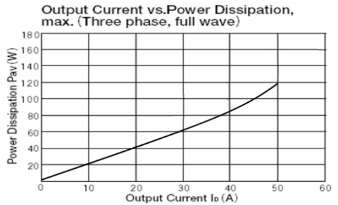
Fig.2. Output Current vs. Power Dissipation
