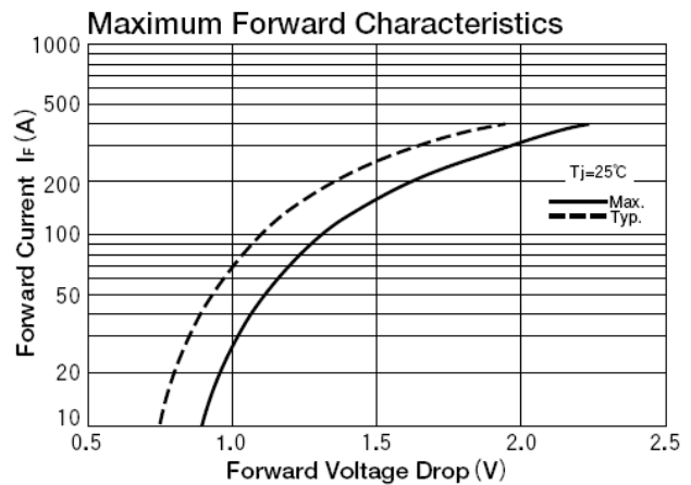
Fig.4. Forward characteristics of a diode
