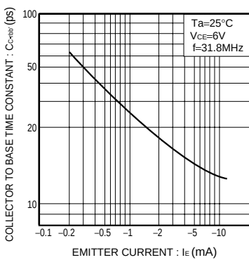
Fig.9 Collector to base time constance vs. emitter current
