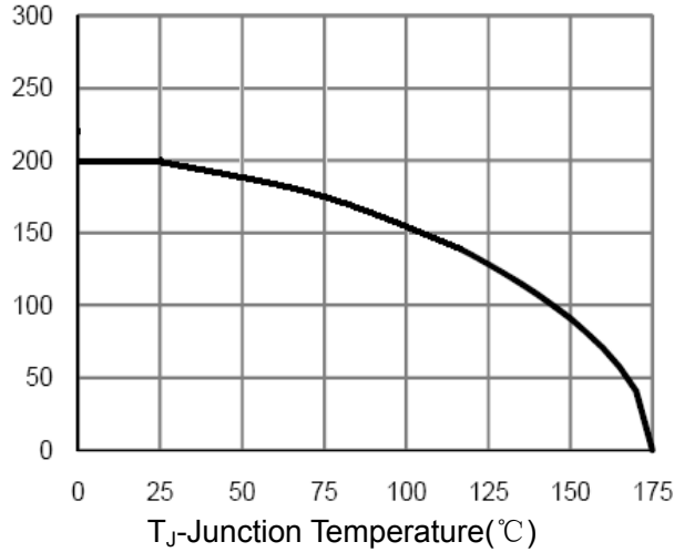
Figure 9 Current De-rating
