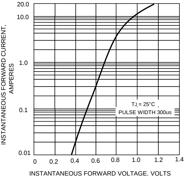
FIG.4-TYPICAL FORWARD CHARACTERISTICS
