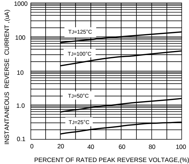
FIG.3-TYPICAL REVERSE CHARACTERISTICS
