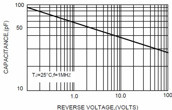
FIG.5-TYPICAL JUNCTION CAPACITANCE
