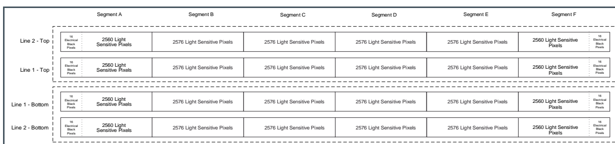
Figure 25: 4LS15K Sensor with Six Stitched 2K5 Segments
