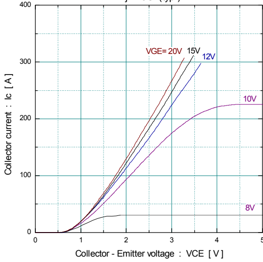
[ Inverter ] Collector current vs. Collector-Emitter voltage T j = 25C (typ.)
