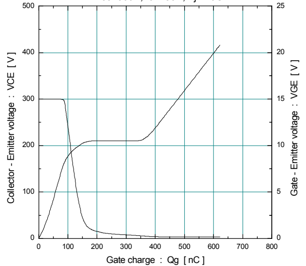
[ Inverter ] Dynamic Gate charge (typ.) Vcc=300V, Ic=150A, Tj= 25C
