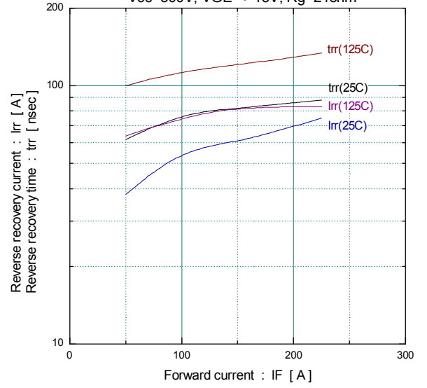
[ Inverter ] Reverse recovery characteristics (typ.) Vcc=300V, VGE=+-15V, Rg=24ohm
