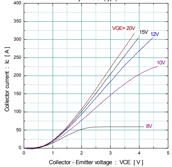
[ Inverter ] Collector current vs. Collector-Emitter voltage T j = 125C (typ.)
